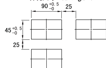
开孔尺寸 Mounting size
